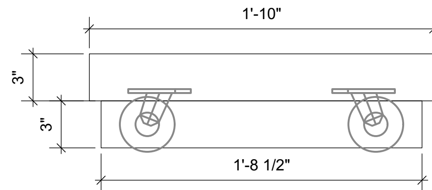
4 FRONT VIEW W/ MOULDING Scale: 2" = 1'-0"
